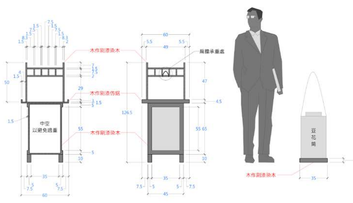
3 豆花攤 SEC SCALE 1:20
